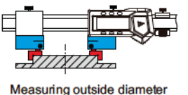
Measuring outside diameter
