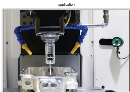
find center of rectangular boss
