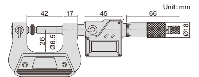
Anvil/spindle tip (included) Unit: mm
