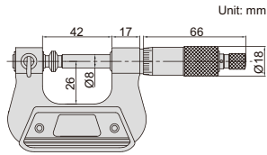
Anvil/spindle tip (included) Unit: mm
